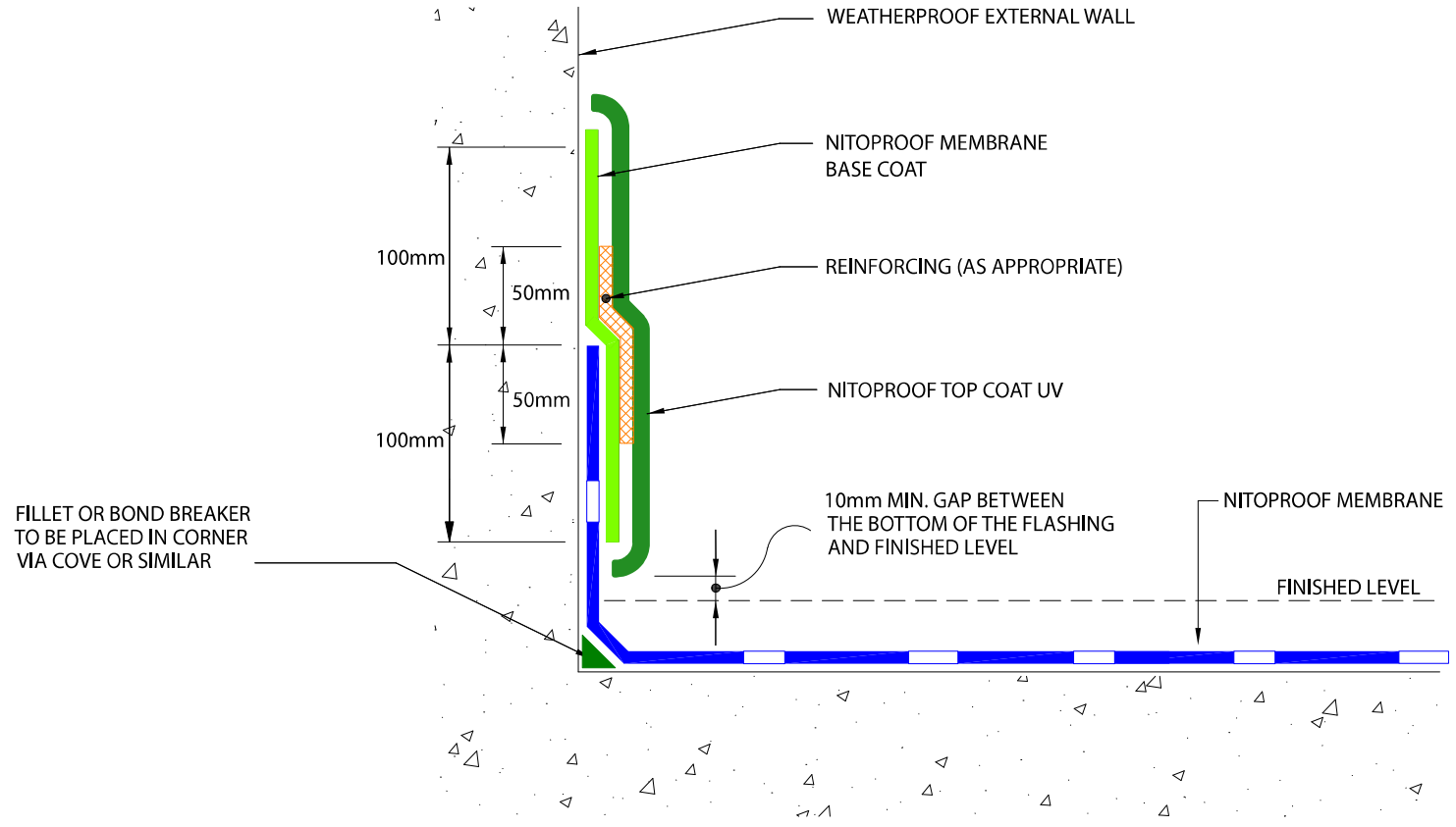
(b) OVERFLASHING CONSTRUCTED OF A LIQUID-APPLIED MEMBRANE
