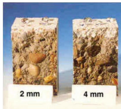
Typical penetration depth of Nitocote SN508 Creme on porous concrete. 0.25 litres/m 2 gave 2 mm penetration. 0.44 litres/m 2 gave 4 mm penetration.
