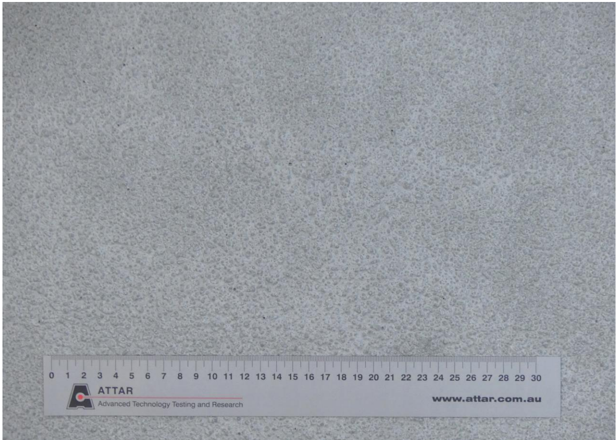
Figure 1: Fosroc Nitoflor PU 600 + Aluminium Oxide (#16) Broadcast + Fosroc Nitoflor PU 200
