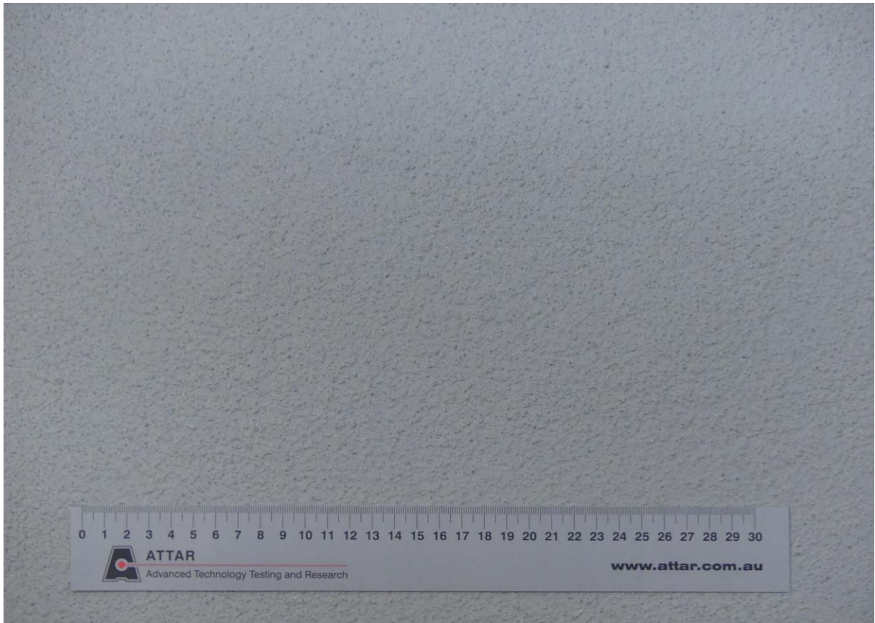
Figure 1: Fosroc Nitoflor PU 600 + Calcined Bauxite (0.5 to 1.0 mm) Broadcast + Fosroc Nitoflor PU 200
