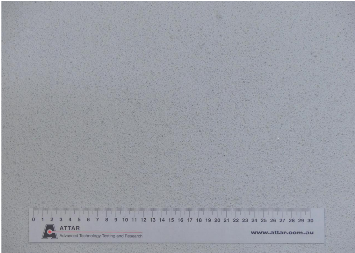
Figure 1: Fosroc Nitoflor PU 600 + Silica Sand (16/30) Broadcast + Fosroc Nitoflor PU 200
